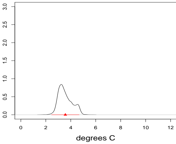
WAF: Delta T, DJF
