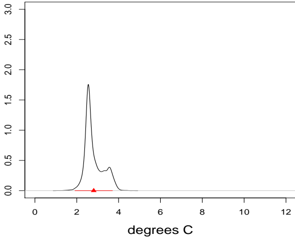
SEA: Delta T, DJF
