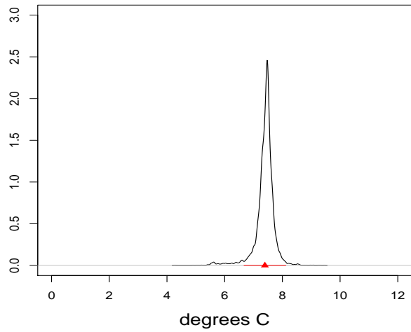
ALA: Delta T, DJF
